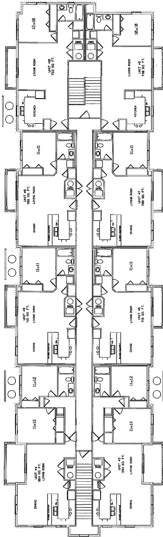
SECOND LEVEL FLOOR PLAN SCALE: 3/16" = 1'-0"
